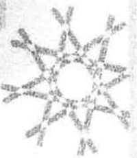
Online Learning
